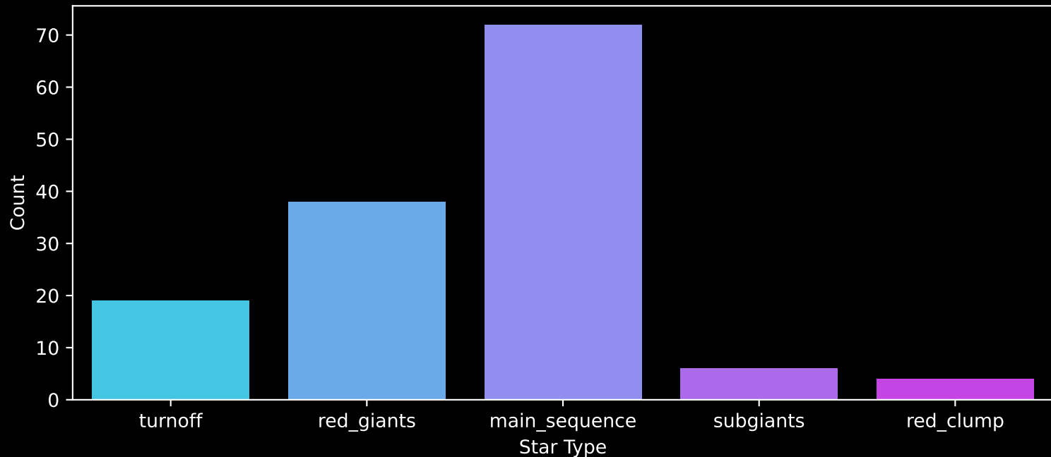
APOGEE DR17 Field: [040+36_MGA] Count plot of Star Type
