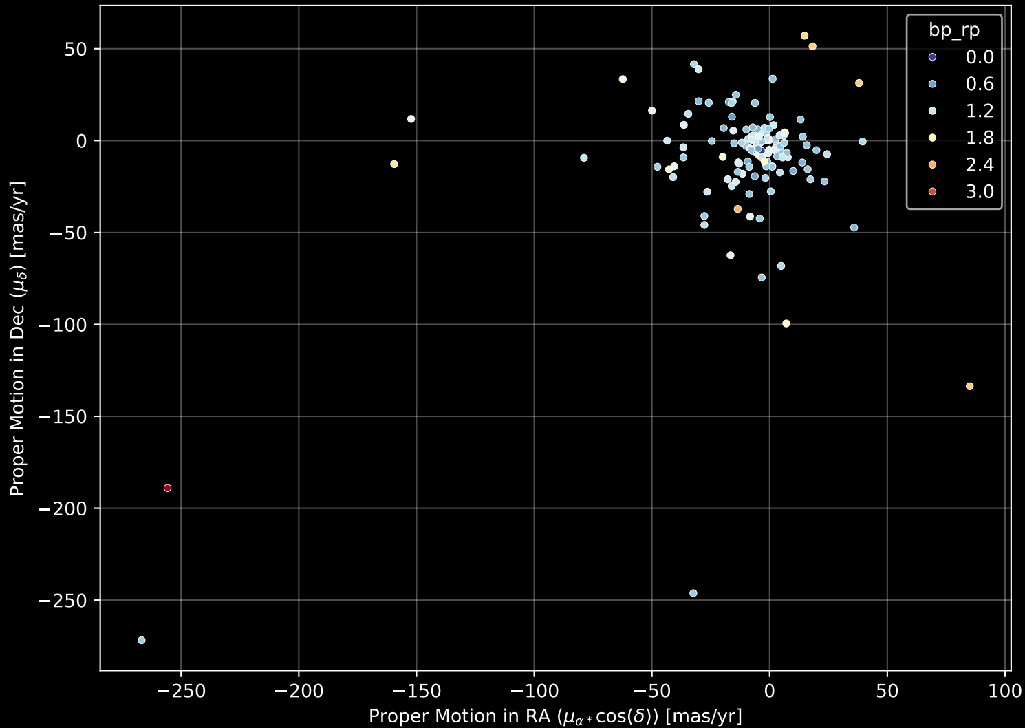
APOGEE DR17 Field: [040+36_MGA] Proper Motion Diagram (n= 139)
