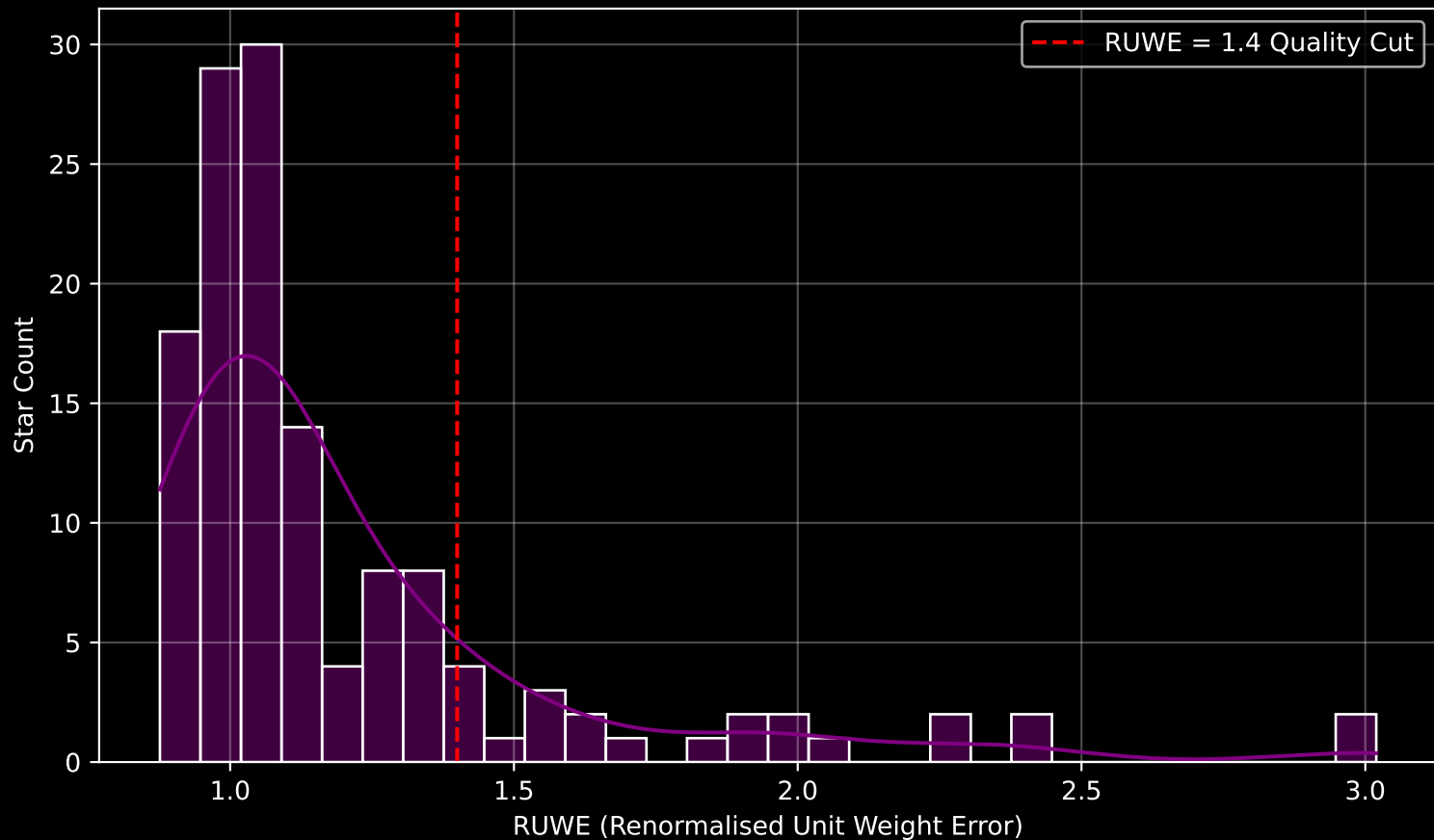
GAPOGEE DR17 Field [040+36_MGA] RUWE Distribution (n= 134)
