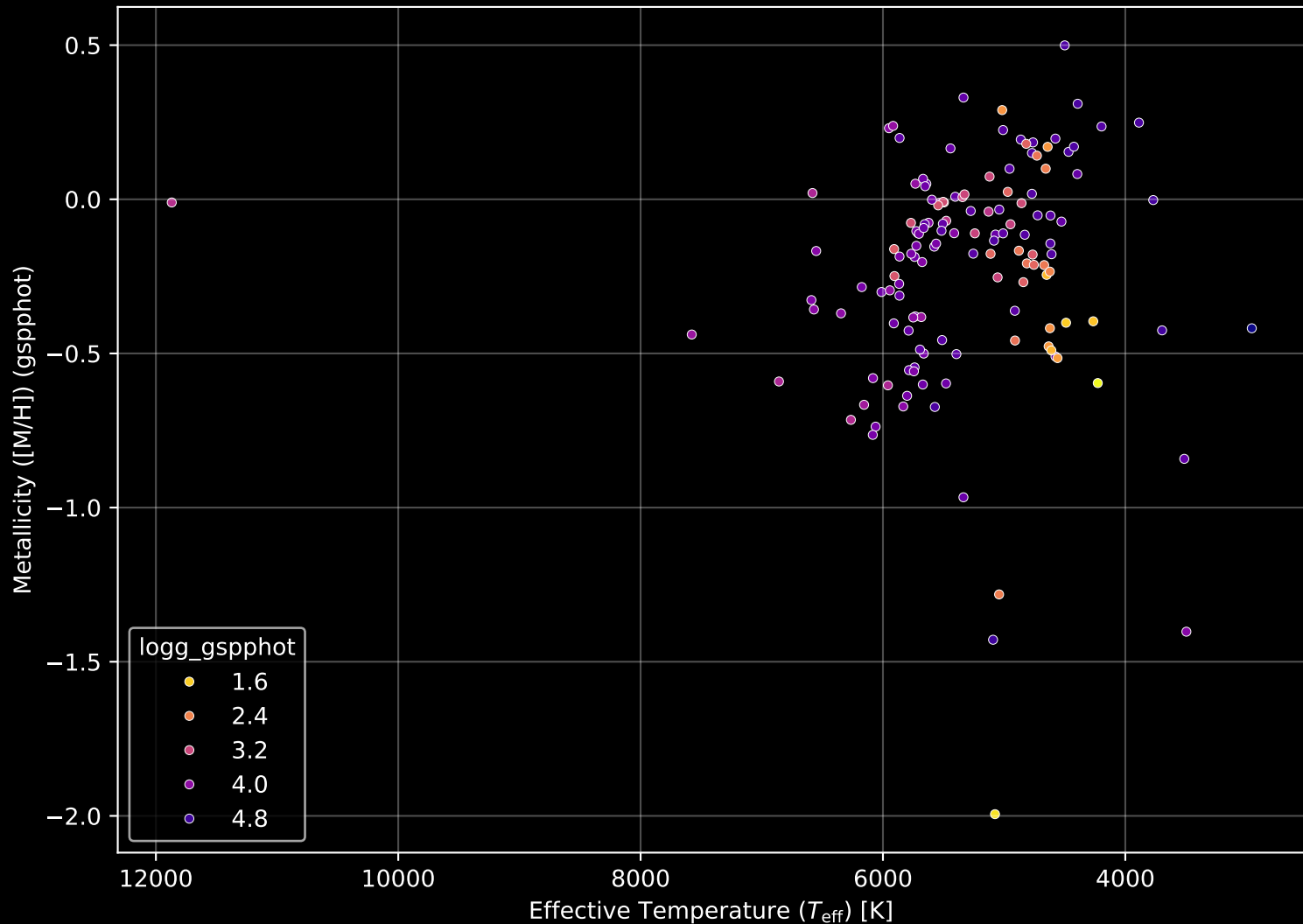
APOGEE DR17 Field: [040+36_MGA] Stellar Population Parameters (n= 139)
