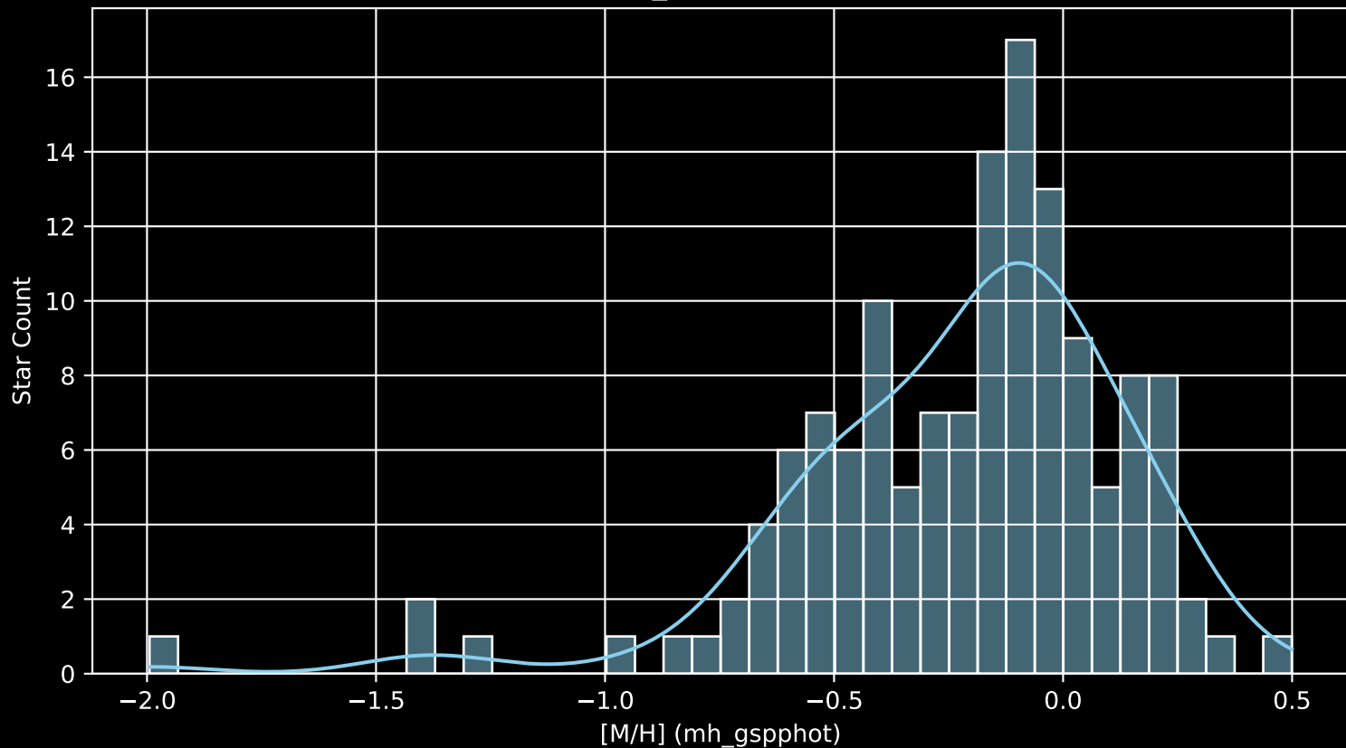
APOGEE DR17 Field: [040+36_MGA [M/H] (mh_gspphot) (n= 139)
