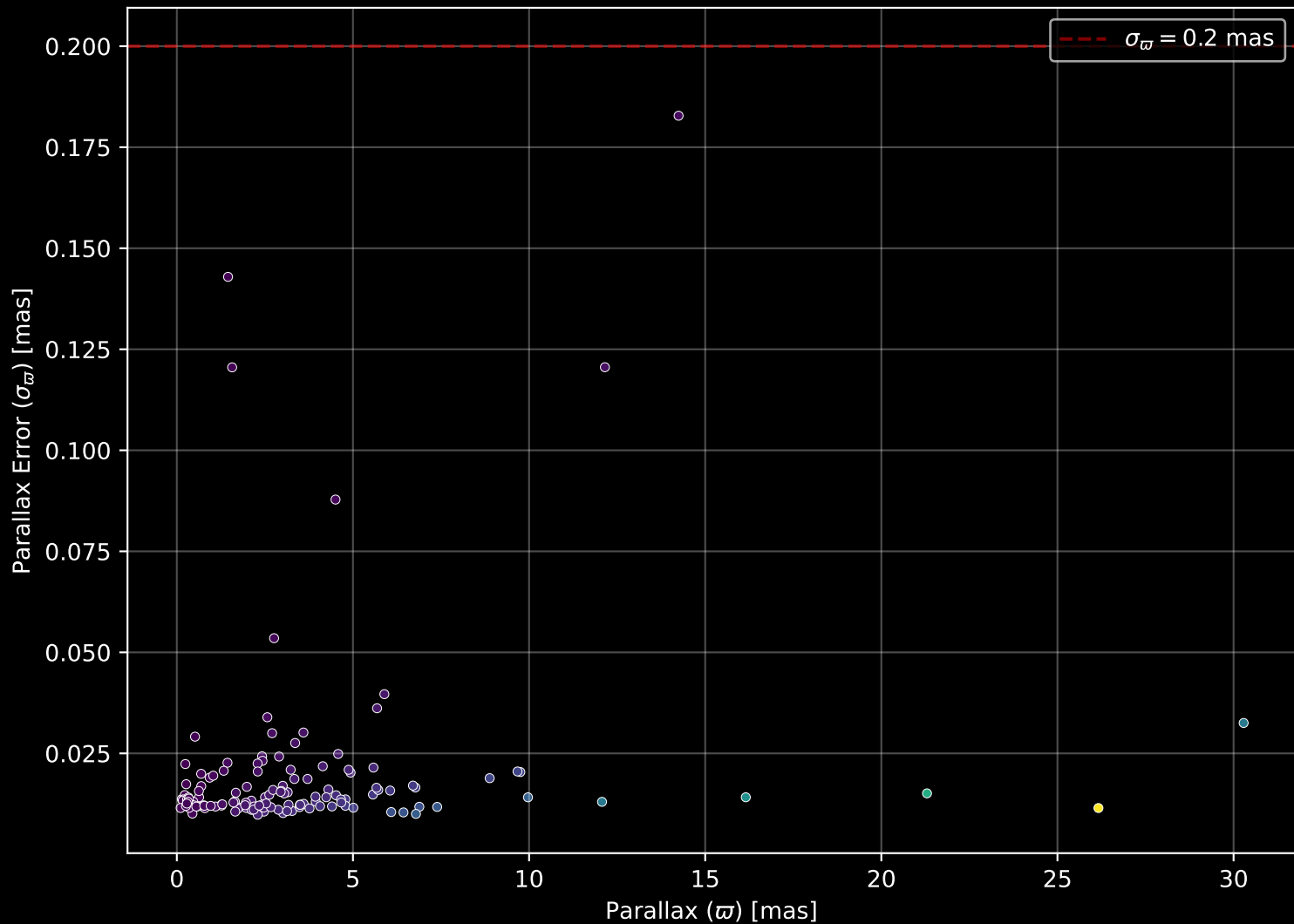
APOGEE DR17 Field: [040+36_MGA] Parallax Quality (n= 139)
